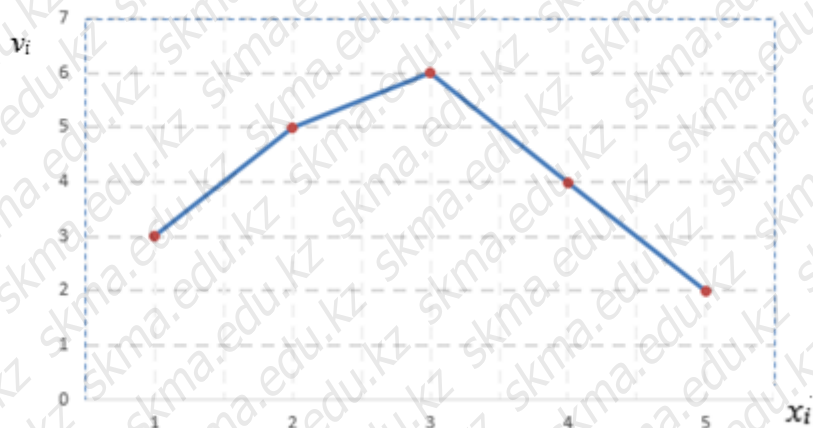
Figure. 2.2. Polygon
